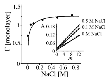
Figure 5. Surface coverage per layer, \Gamma , of Eu-POM in (Eu-POM/PAH) m multilayers as a function of the NaCl concentration of the Eu-POM solution. The surface coverage is based on the packing density in the crystalline solid. PAH is deposited from aqueous solution containing no NaCl. The inset shows the absorbance at 282 nm at different NaCl concentrations versus the number of layers, m , confirming linear multilayer growth.
